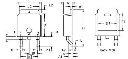
TO-252 AA (IXTY)
