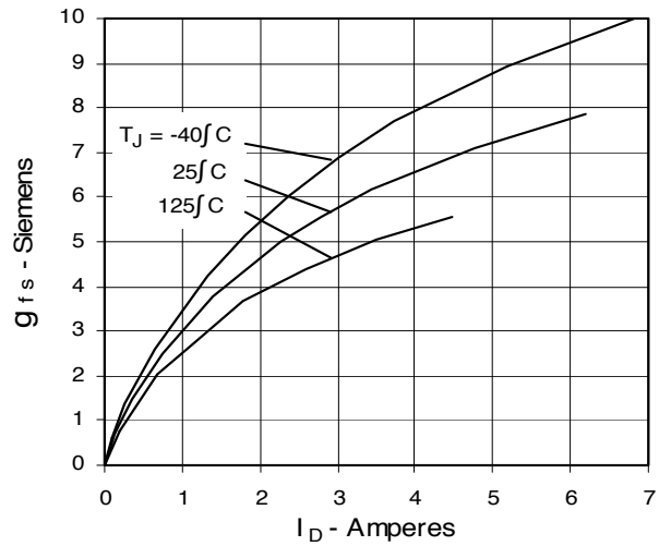
Fig. 8. Transconductance
