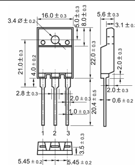
TO-3PML
