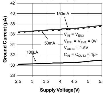
Ground Current vs Supply Voltage (single output)
