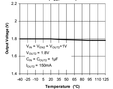
Output Voltage vs Temperature ( V_{OUT} = 1.8V )
