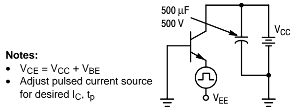
Figure 19. Overload SOA Test Circuit
