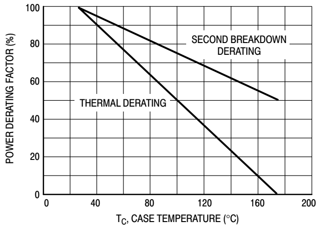
Figure 15. Power Derating
