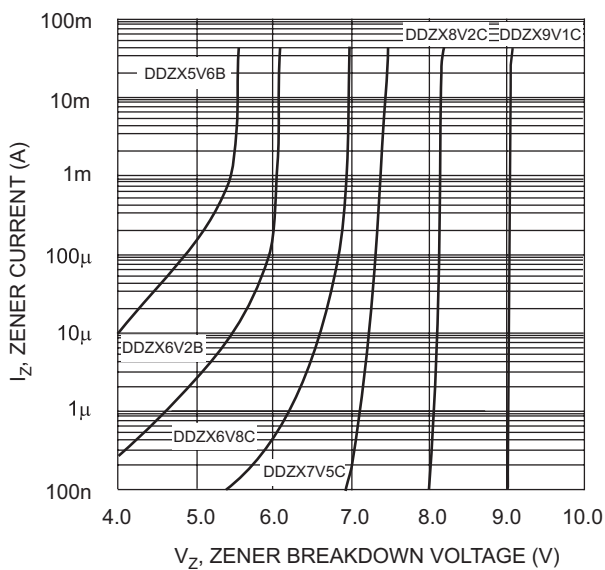
Fig. 4 Typical Reverse Characteristics, DDZX5V6B - DDZX9V1C
