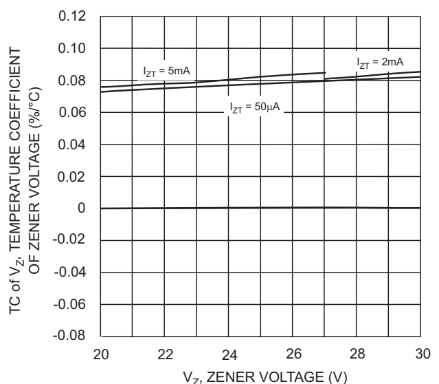
Fig. 17 Typical Temperature Coefficient of Zener Voltage vs. Zener Voltage, DDZX20C-DDZX30D
