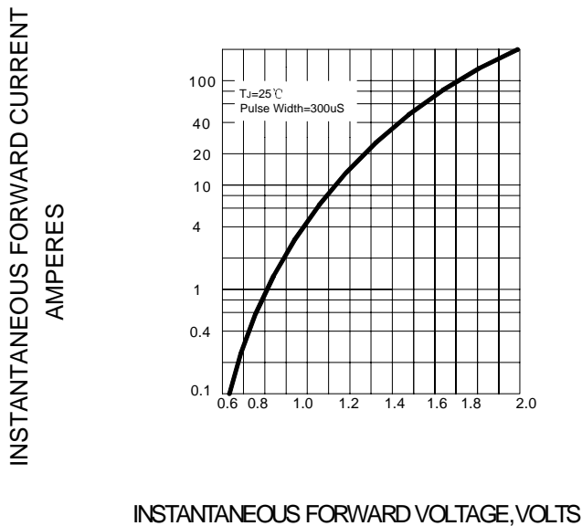
FIG.4–TYPICAL FORWARD CHARACTERISTIC
