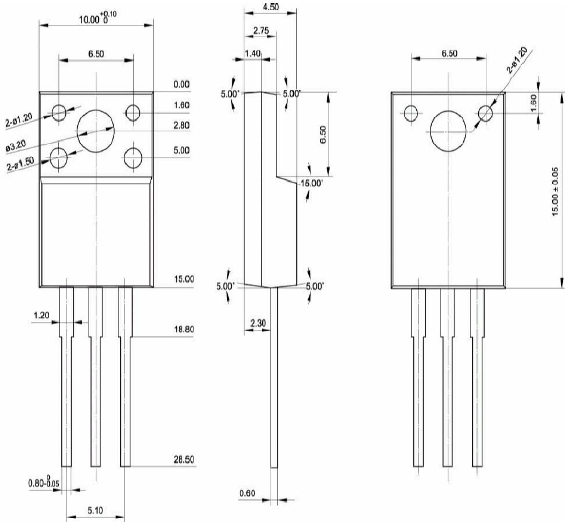
Fig.2 Outline dimensions (unindicated tolerance: \pm 0.10 mm)
