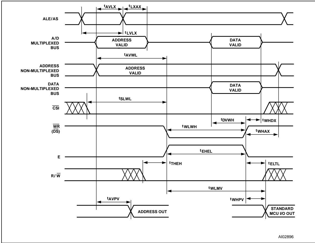
Figure 46. WRITE Timing
