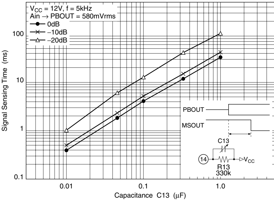
Signal Sensing Time vs. Capacitance
