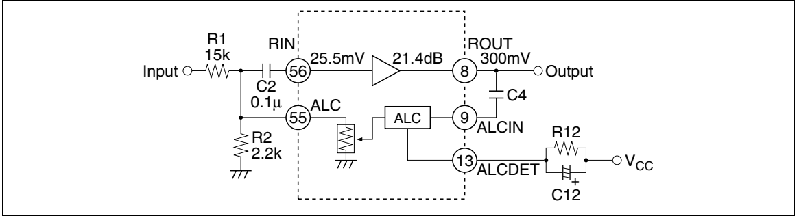
Figure 12 ALC Block Diagram
