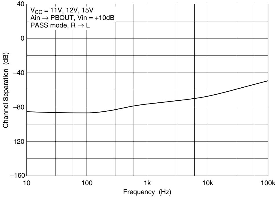
Channel Separation vs. Frequency (R → L) (7)
