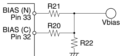
Figure 10 External Components of Bias Block
