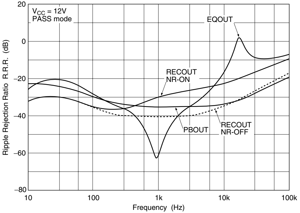
Ripple Rejection Ratio vs. Frequency (PASS mode) (3)
