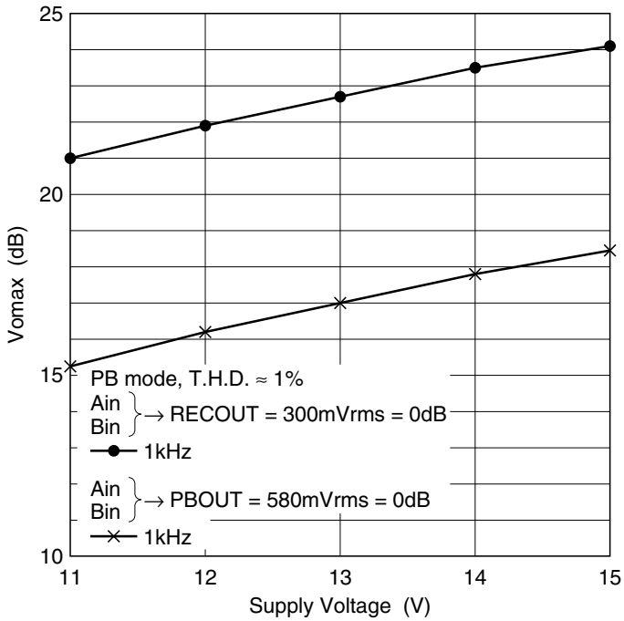
Signal Handling (2)
