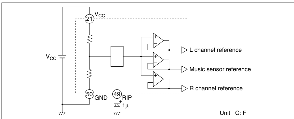
Figure 1 Reference Voltage
