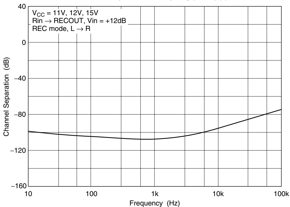
Channel Separation vs. Frequency (L → R) (2)
