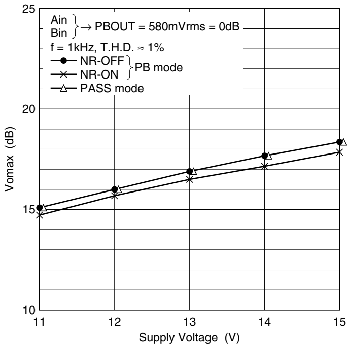
Signal Handling (2)
