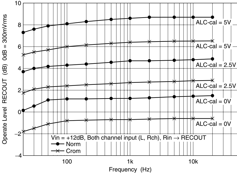
ALC Operate Level vs. Frequency
