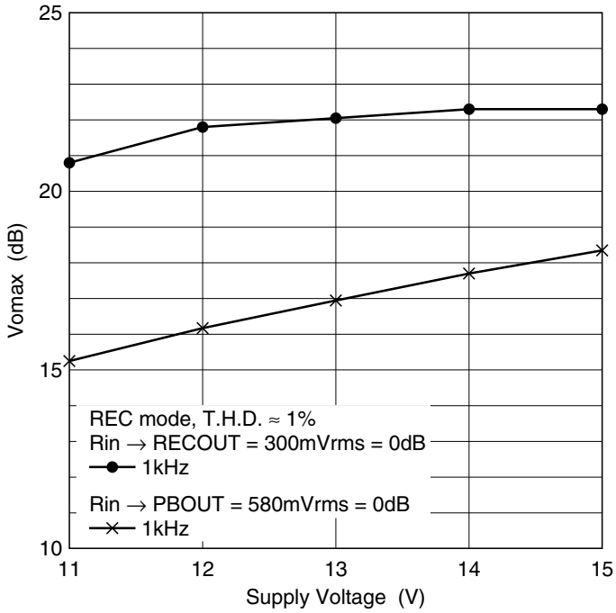
Signal Handling (1)
