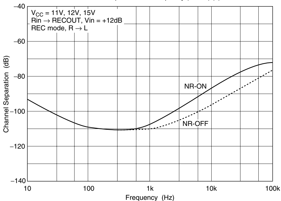
Channel Separation vs. Frequency (R → L) (1)
