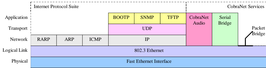
Figure 6. CobraNet Network Stack
