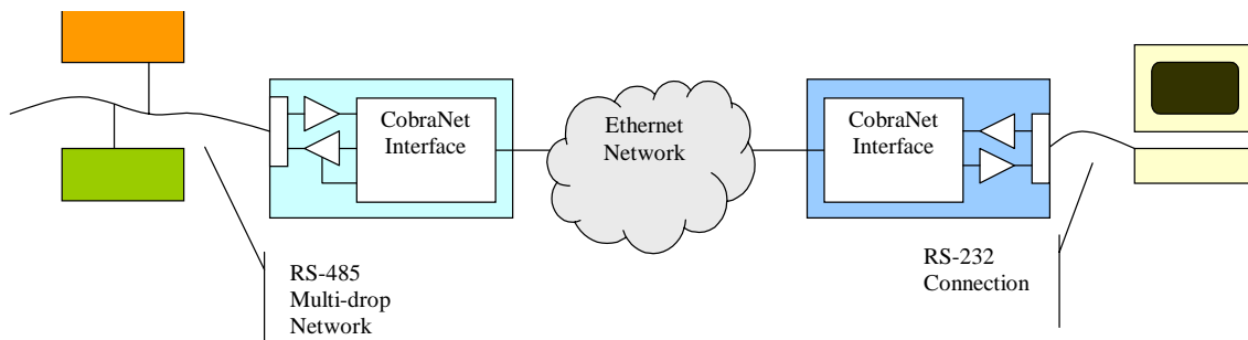
Figure 2. Serial Bridging, External Application
