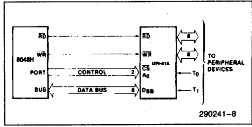
Figure 2. 8048-8741A Interface
