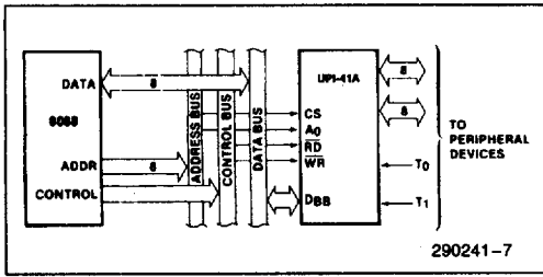
Figure 1. 8085A-8741A Interface
