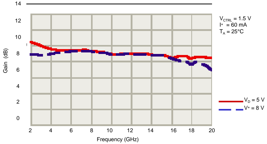
TYPICAL SMALL SIGNAL POWER GAIN
