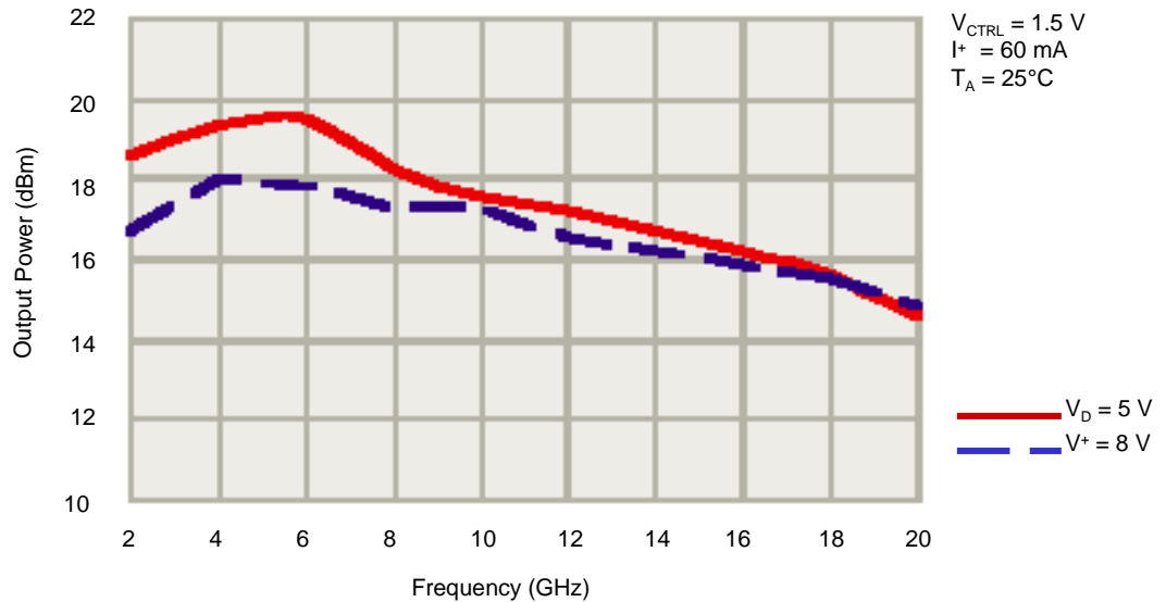
TYPICAL OUTPUT POWER P1dB
