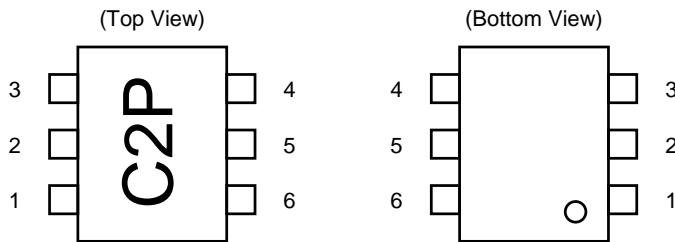
Marking is an example of \mu PC8128TB
