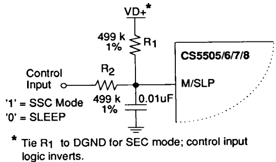
Figure 13. Sleep Threshold Control
