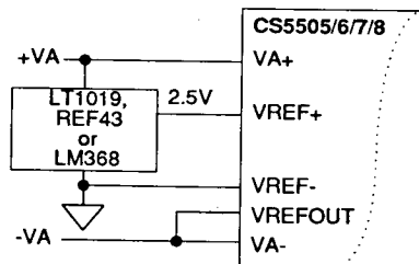
Figure 5. External Reference Connections
