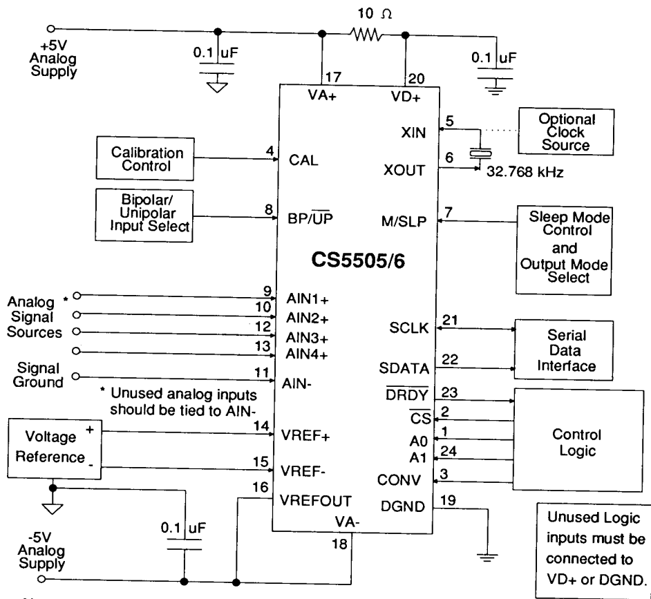
Figure 14. CS5505/6 System Connection Diagram Using External Reference, Dual Supplies
