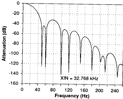
Figure 9. Filter Magnitude Plot to 260 Hz
