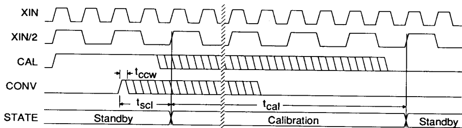
Figure 1. Calibration Timing (Not to Scale)
