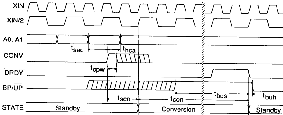
Figure 2. Conversion Timing (Not to Scale)
