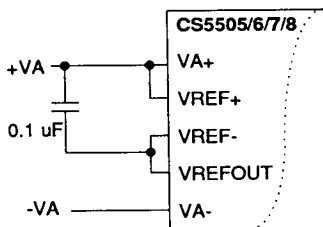
Figure 6. Internal Reference Connections
