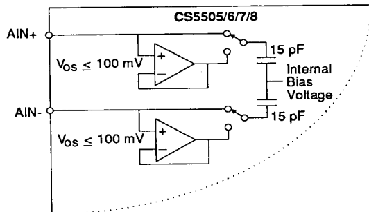
Figure 8. Analog Input Model
