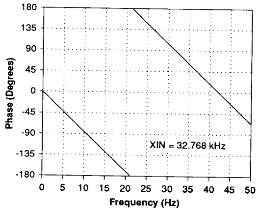
Figure 11. Filter Phase Plot to 50 Hz
