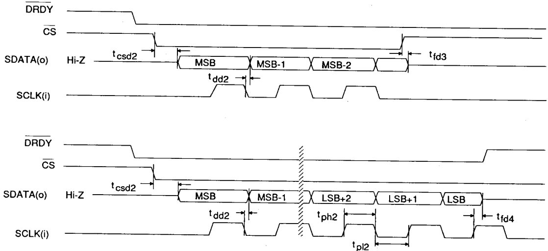
Figure 4. Timing Relationships; SEC Mode (Not to Scale)
