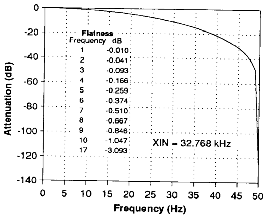
Figure 10. Filter Magnitude Plot to 50 Hz
