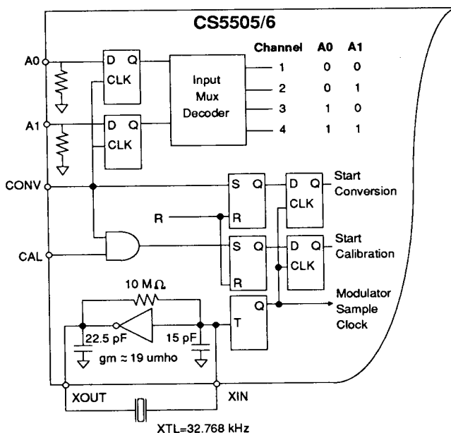
Figure 12. Gate Oscillator and Control Logic
