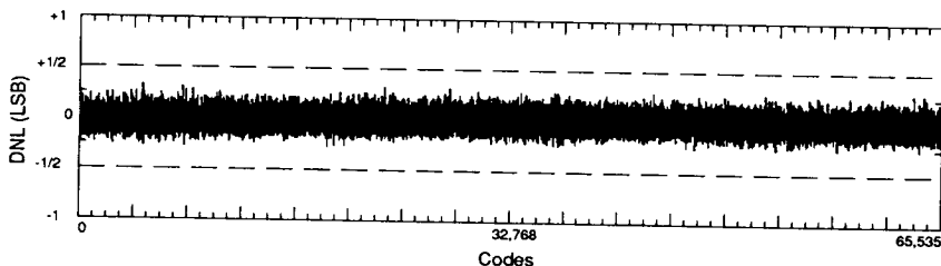
Figure 7. CS5505 Differential Nonlinearity plot.
