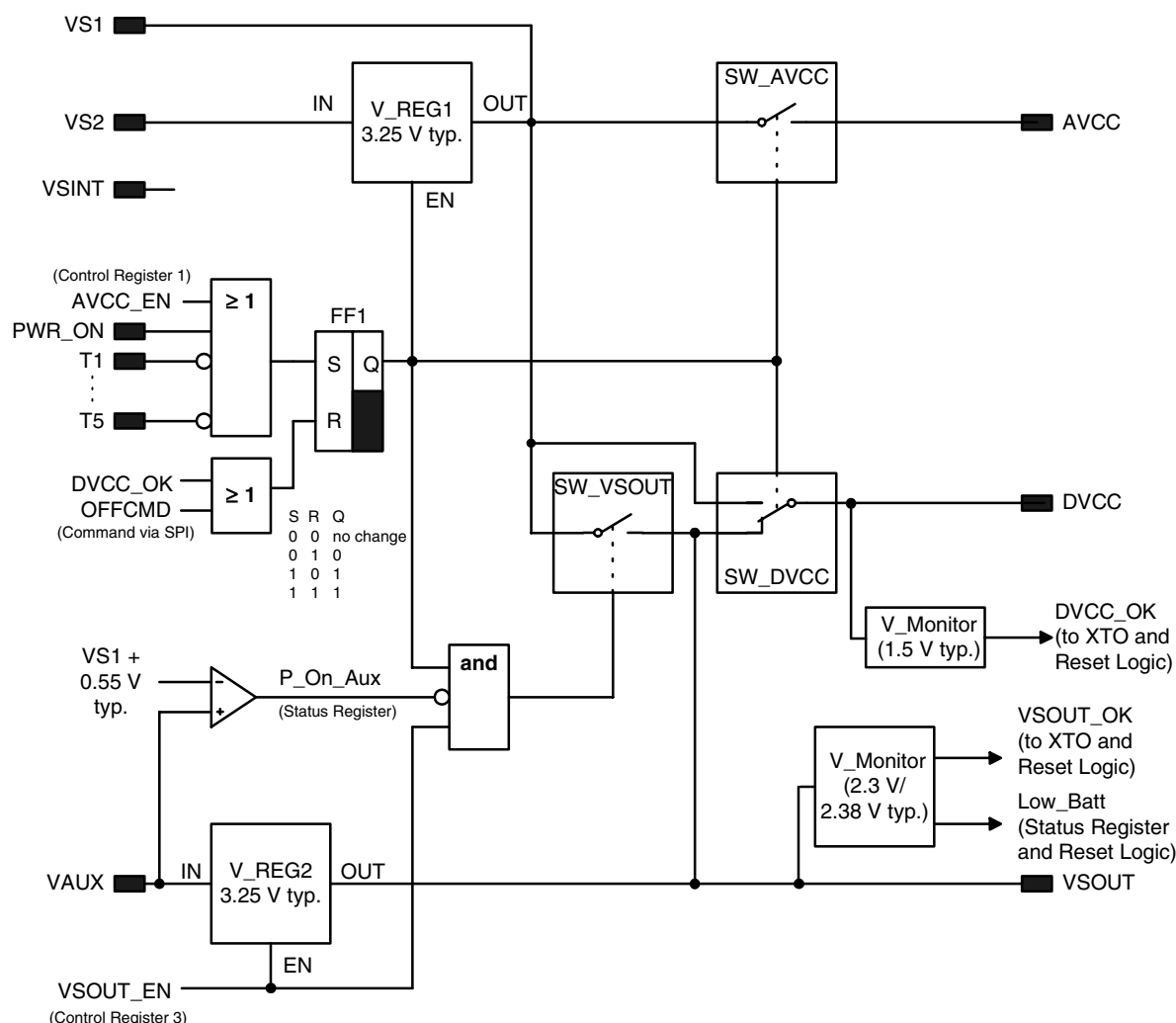
Figure 5-1. Power Supply
