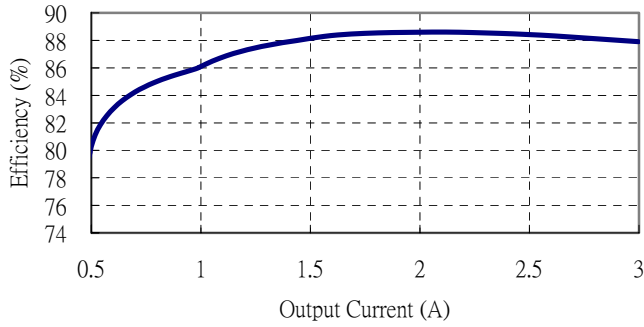
Figure 3: Converter efficiency vs. output current (12V in, 2.5V output voltage)
