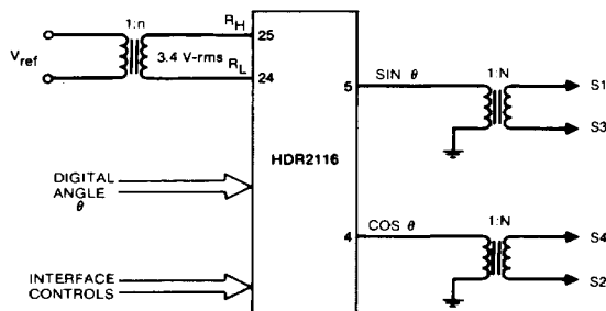
FIGURE 11 Digital-to-Resolver Converter
