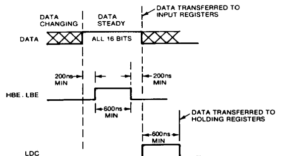
FIGURE 7 Single-Byte Loading
