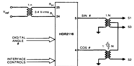
FIGURE 12 Digital-to-Synchro Converter
