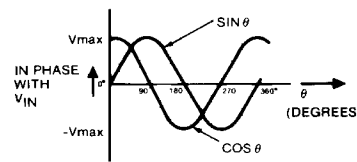
FIGURE 10 Output Phasing
