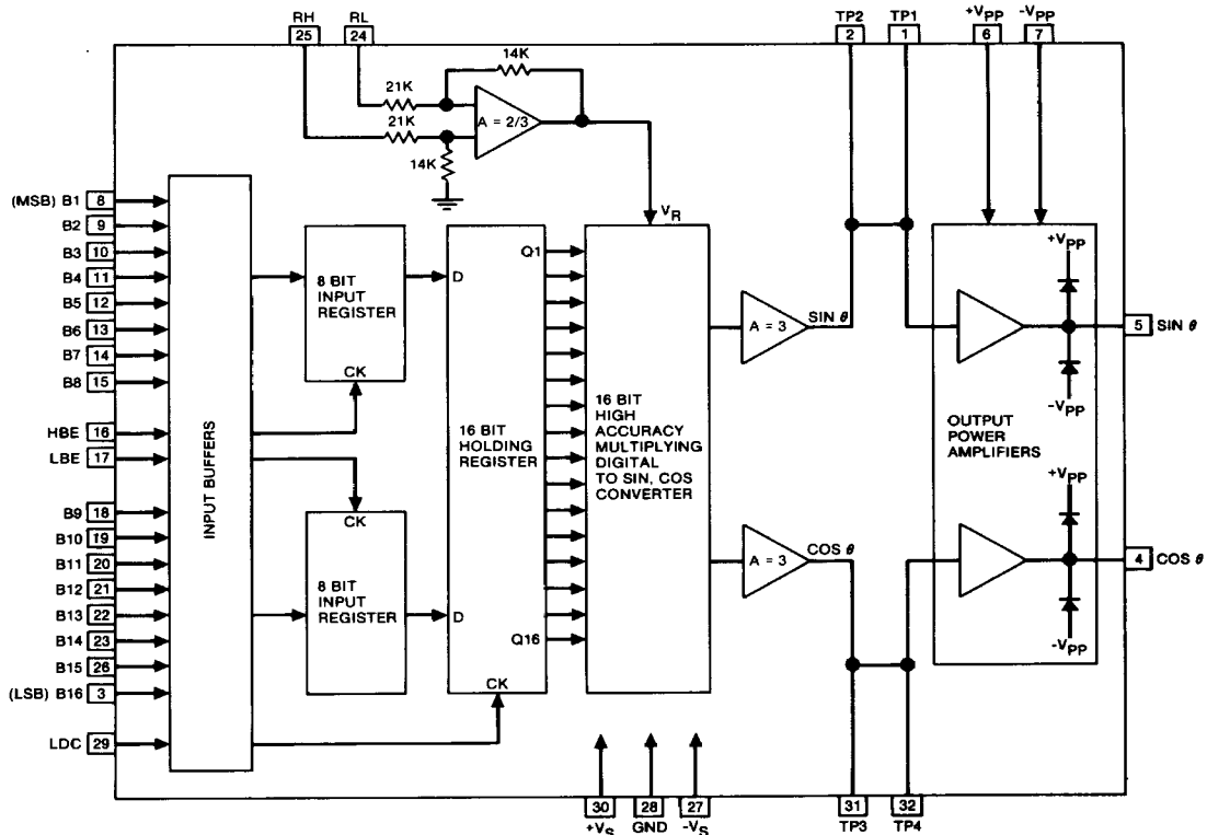
FIGURE 1 2116 Block Diagram
