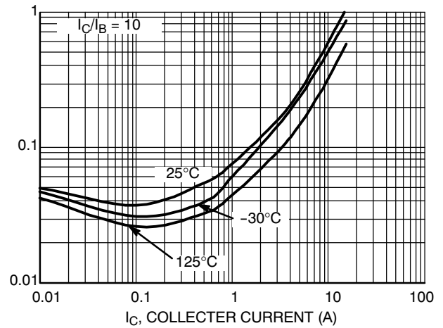
Figure 10. V_{CE(sat)} , Collector-Emitter Saturation Voltage
