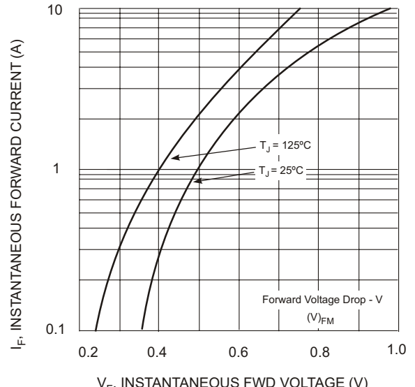
V_F , INSTANTANEOUS FWD VOLTAGE (V) Fig. 2 Typ. Forward Characteristics
