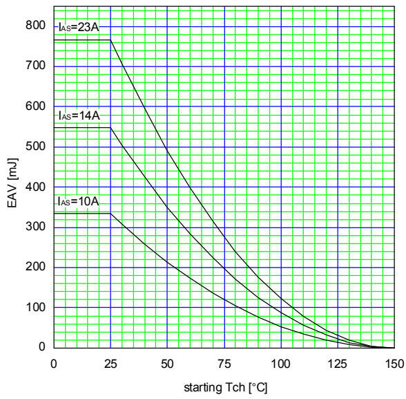
Maximum Avalanche Energy vs. starting Tch E(AV)=f(\text{starting Tch}):V_{CC}=50V, I(AV)\leq 23A
