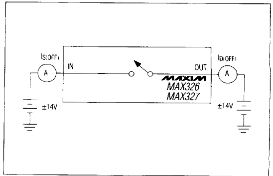
Figure 5. Off Leakage Current Test Circuit
