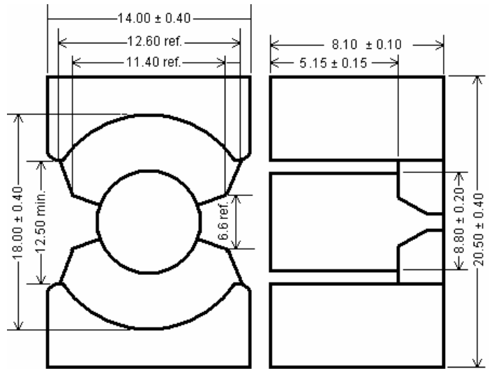
Dimensions (mm)
