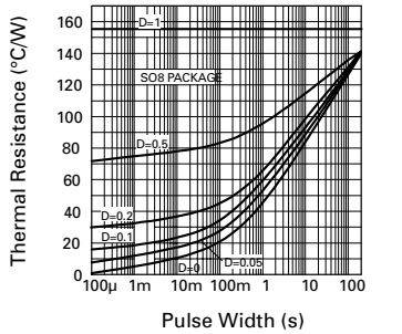
Thermal Resistance v Pulse Width
