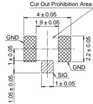
Recommended PCB Footprints
