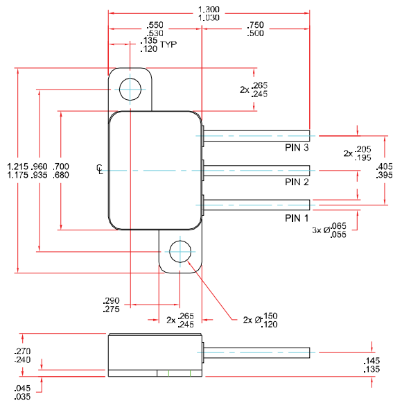
Case Outline: TO-259
