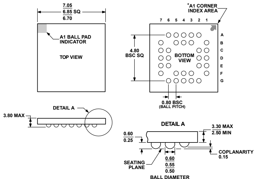
Figure 24. 32-Lead Ceramic Ball Grid Array [CBGA] (BG-32-3) Dimensions shown in millimeters
