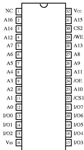
(Top View)
