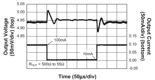
Load Transient Response (10mA - 100mA; V_{IN} = 3.3V )
