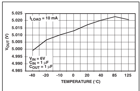
FIGURE 2-12: Output Voltage (5V) vs. Temperature ( I_{LOAD} = 10 \text{ mA} ).
