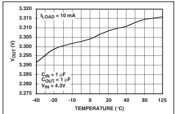
FIGURE 2-11: Output Voltage (3.3V) vs. Temperature ( I_{LOAD} = 10 \text{ mA} ).
