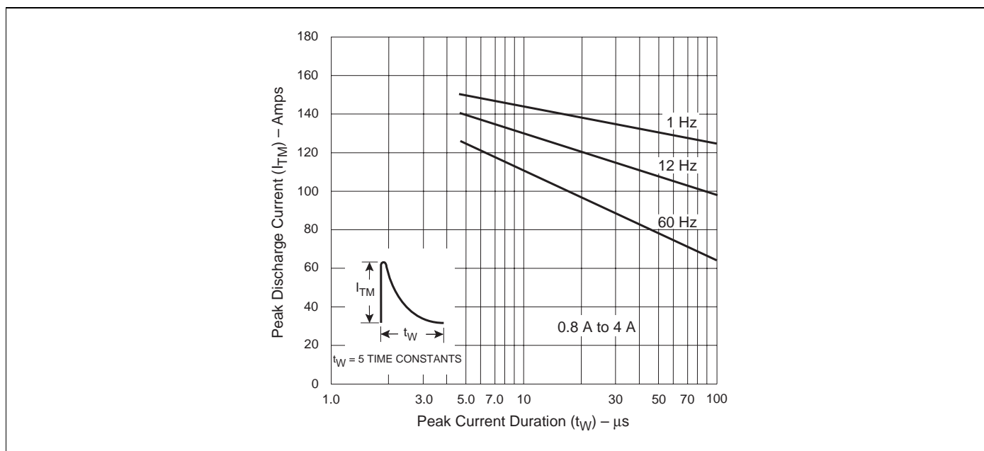
Figure E5.20 Peak Repetitive Capacitor Discharge Current
