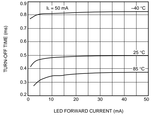
B. Turn-Off Time vs. LED Current (LH1531)
