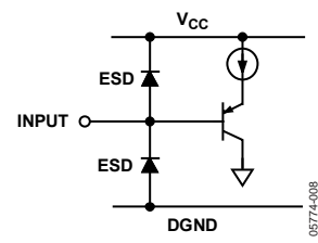
Figure 9. Logic Input
