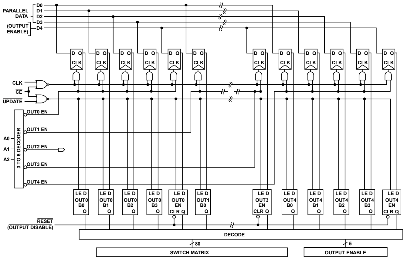
Figure 4. Logic Diagram
