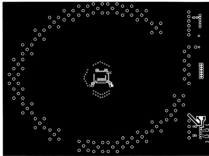
Figure 54. Board Layout (Bottom Layer)
