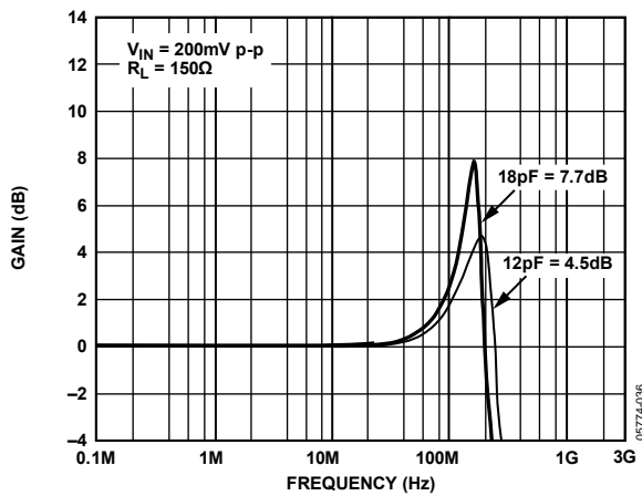
Figure 35. AD8106 Frequency Response vs. Capacitive Load
