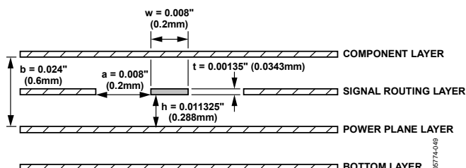
Figure 48. Cross Section of Input and Output Traces
