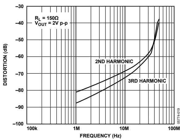
Figure 18. AD8107 Distortion vs. Frequency
