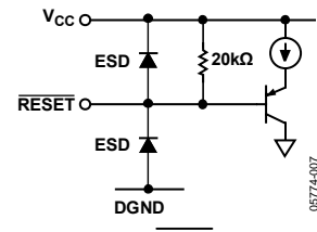
Figure 8. RESET Input
