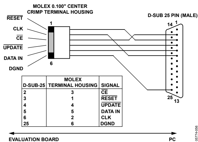
Figure 55. Evaluation Board PC Connection Cable
