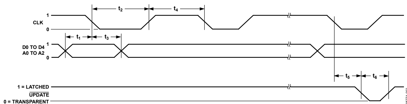
Figure 2. Timing Diagram
