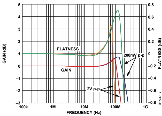
Figure 16. AD8107 Frequency Response
