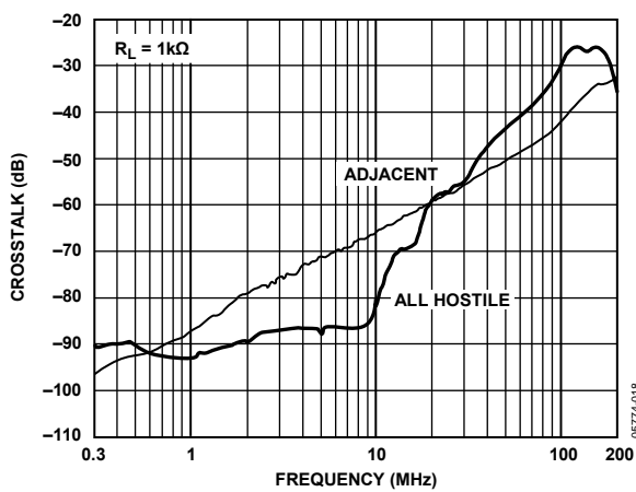
Figure 17. AD8107 Crosstalk vs. Frequency
