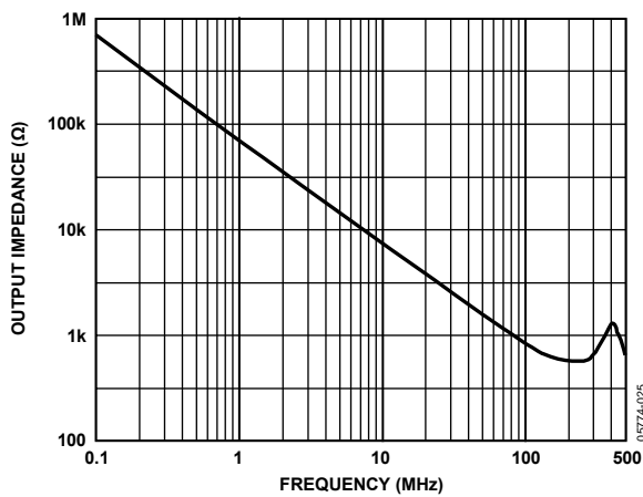
Figure 24. AD8106 Output Impedance, Disabled
