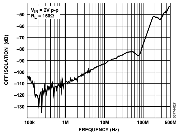
Figure 26. AD8106 Off Isolation, Input/Output
