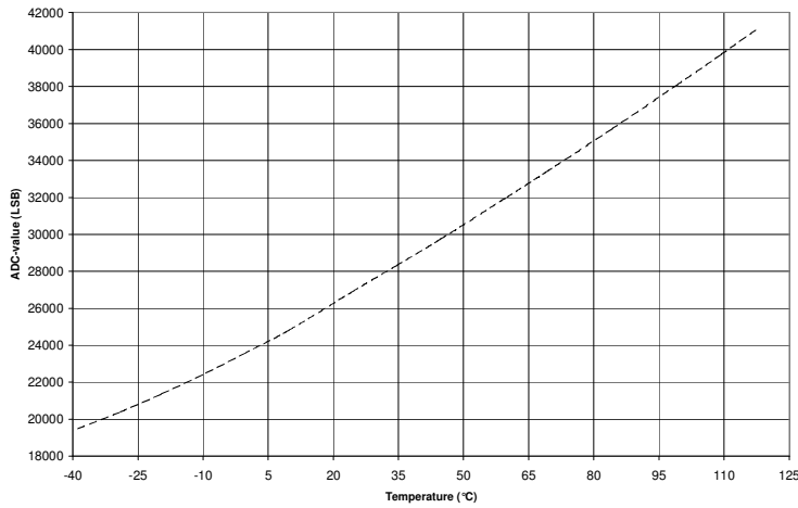
ADC-value D2 vs Temperature (typical)
