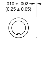
Keyed Washer
