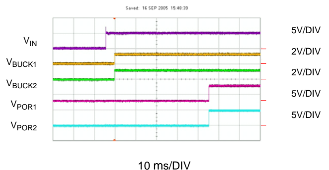
Figure 19: Hot Plug
