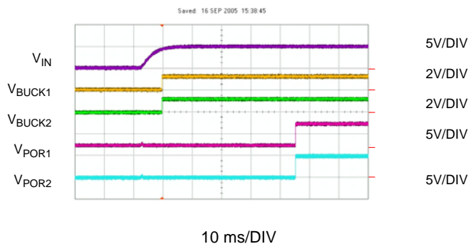
Figure 18: Startup Sequence
