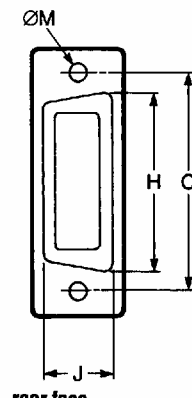
rear face
