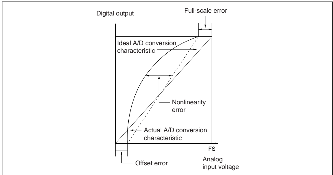
Figure 21.6 A/D Conversion Accuracy Definitions
