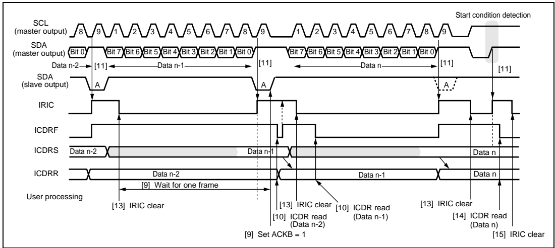
Figure 16.23 Example of Slave Receive Mode Operation Timing (2) (MLS = ACKB = 1)
