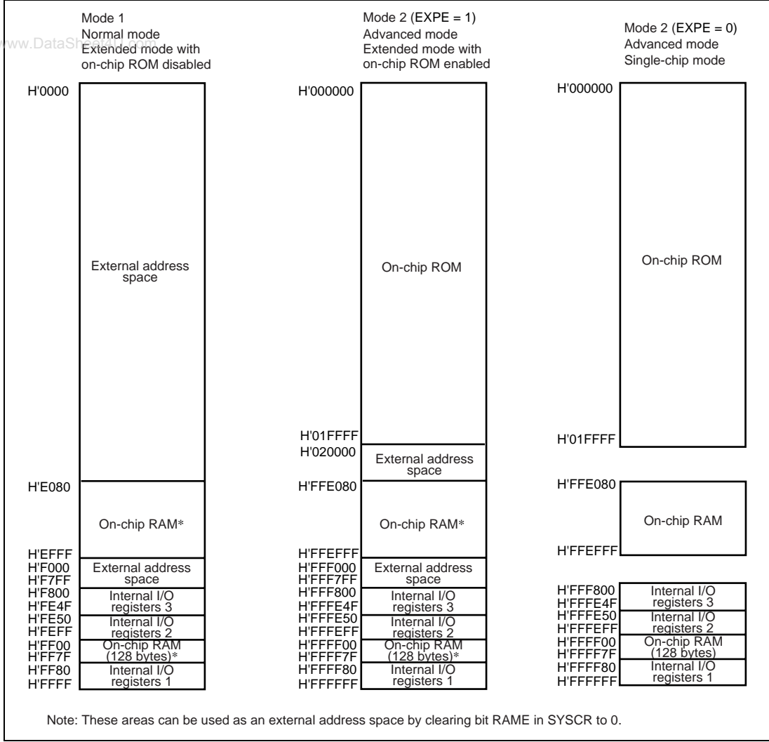
Figure 3.3 Address Map for H8S/2141B and H8S/2161B (1)
