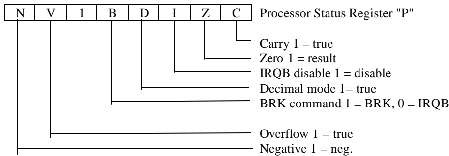
Figure 2-2 W65C02S Microprocessor Programming Model
