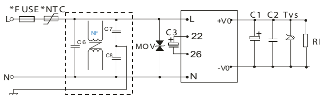
Figure 2 VSK-S3 EMC Application Figure
