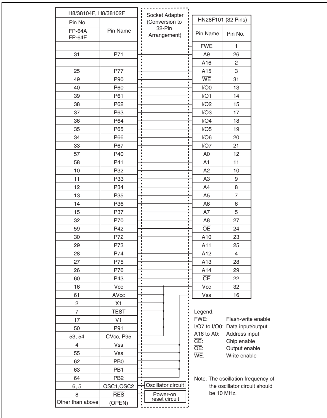
Figure 6.12(2) Socket Adapter Pin Correspondence Diagram (H8/38104F, H8/38102F)
