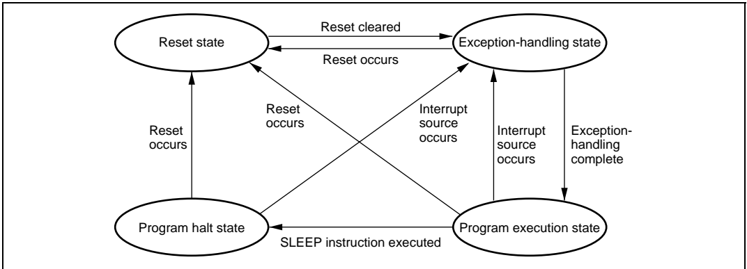
Figure 2.16 State Transitions
