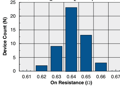
Typical On-Resistance Distribution (N=50, T A =25°C, I L =1A, I F =10mA)
