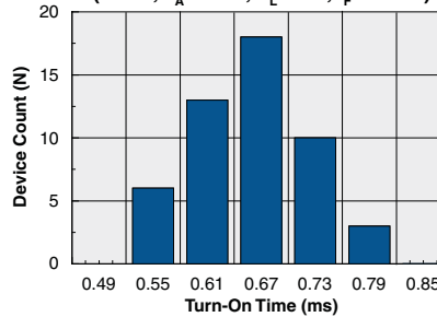
Typical Turn-On Time Distribution (N=50, T A =25°C, V L =10V, I F =10mA)
