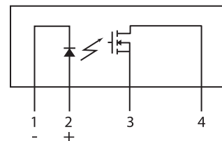
CPC1726 Pinout
