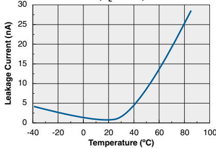
Typical Leakage Current vs. Temperature Measured Across Pins 3 & 4 (V L =250V)
