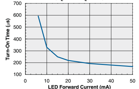
Typical Turn-On Time vs. LED Forward Current (V L =10V, R L =1kΩ)
