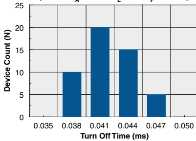
Typical Turn-Off Time Distribution (N=50, T A =25°C, V L =10V, I F =10mA)
