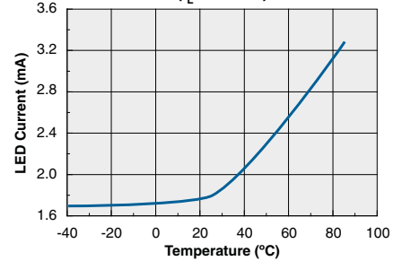
Typical I_F for Switch Operation vs. Temperature ( I_L=500mA )
