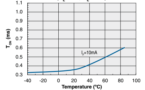
Typical Turn-On Time vs. Temperature (V L =10V, R L =1kΩ)
