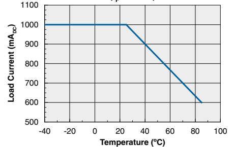
Typical Load Current vs. Temperature (I F =10mA)
