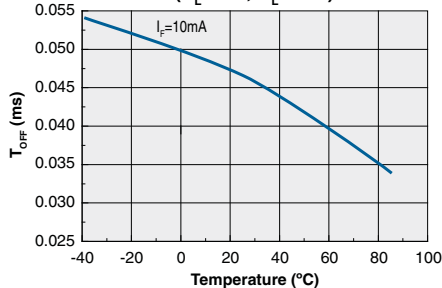
Typical Turn-Off Time vs. Temperature (V L =10V, R L =1kΩ)
