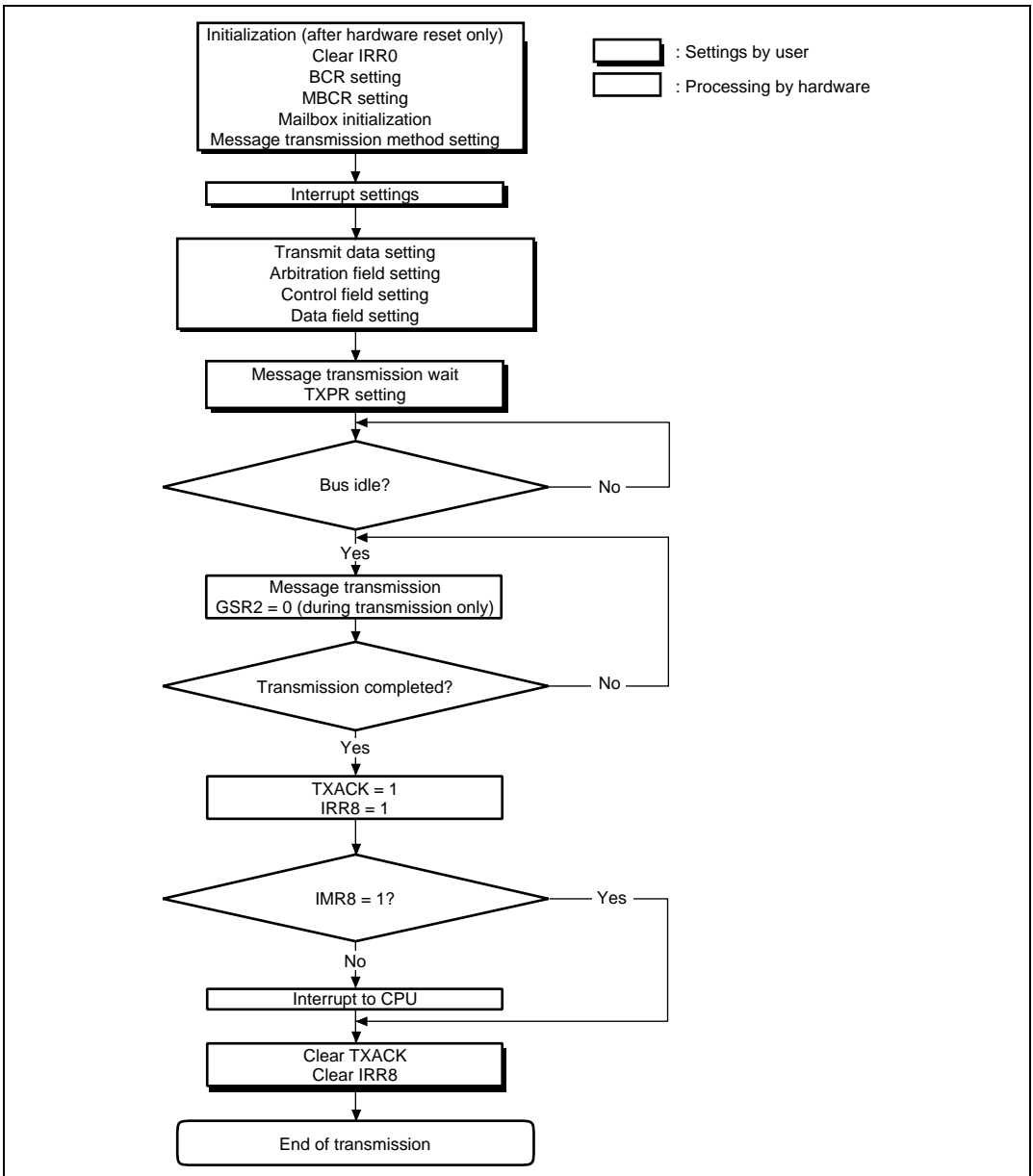
Figure 15.9 Transmission Flowchart
