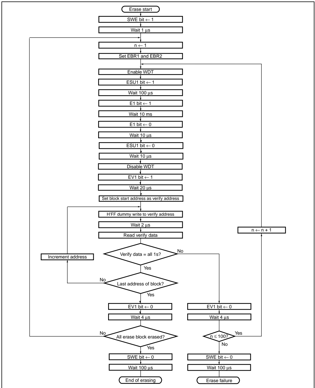
Figure 19.10 Erase/Eraser-Verify Flowchart
