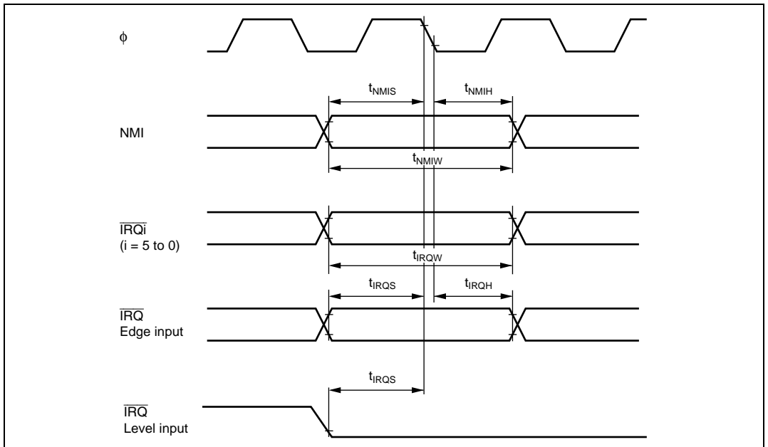
Figure 23.5 Interrupt Input Timing
