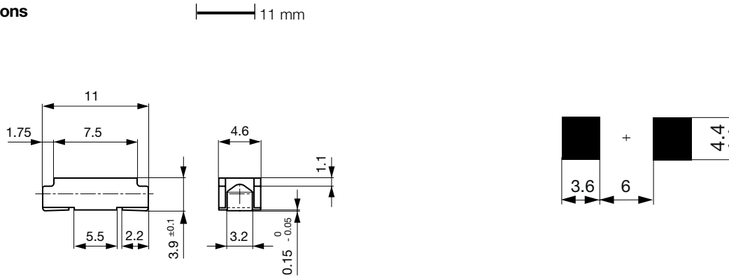
Soldering pads
