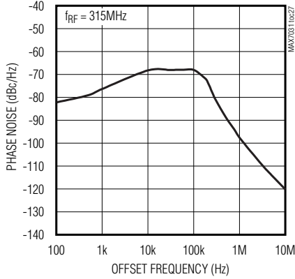
PHASE NOISE vs. OFFSET FREQUENCY (TRANSMIT MODE)
