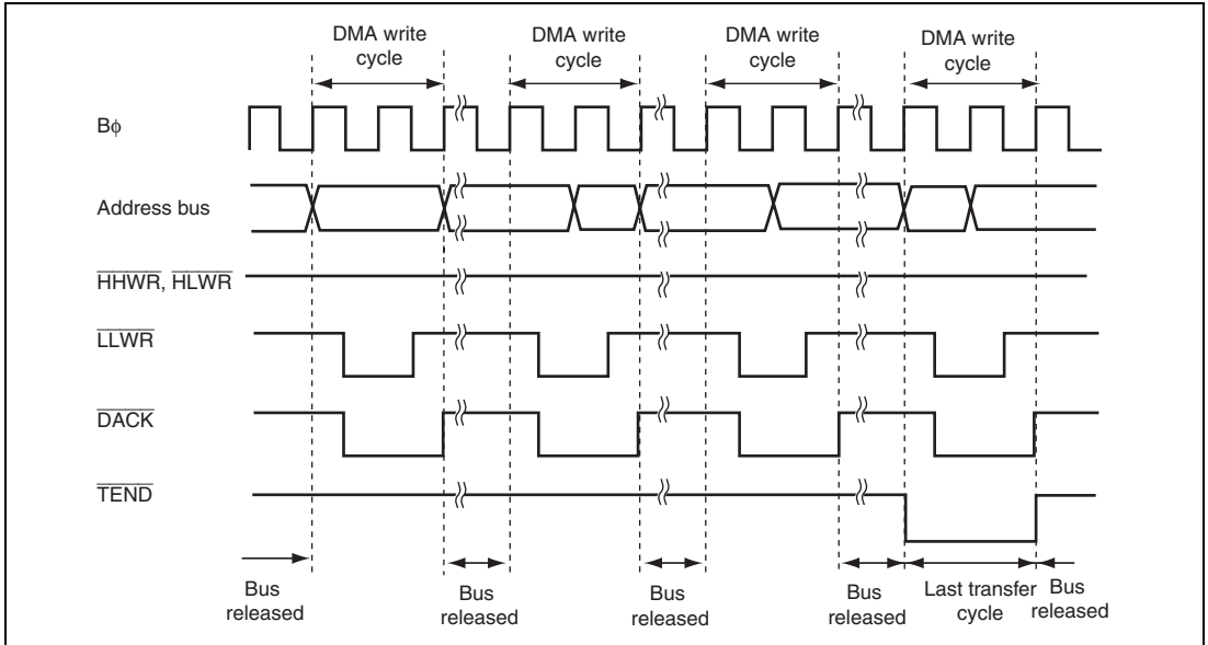
Figure 7.34 Example of Transfer in Single Address Mode (Byte Write)
