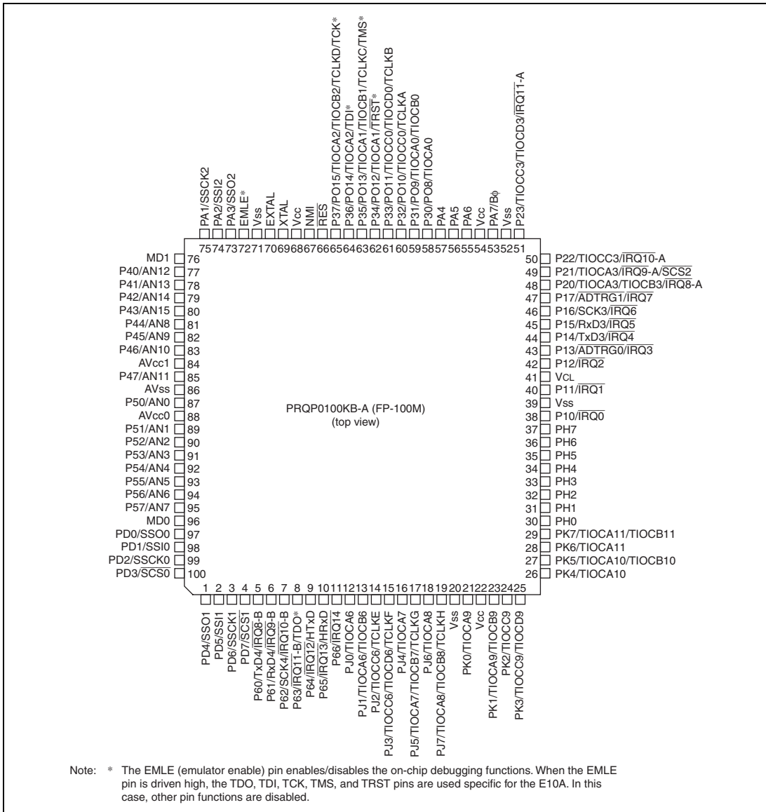
Figure 1.3 Pin Assignments of H8SX/1527
