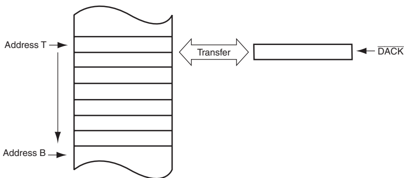
Figure 7.6 Operations in Single Address Mode
