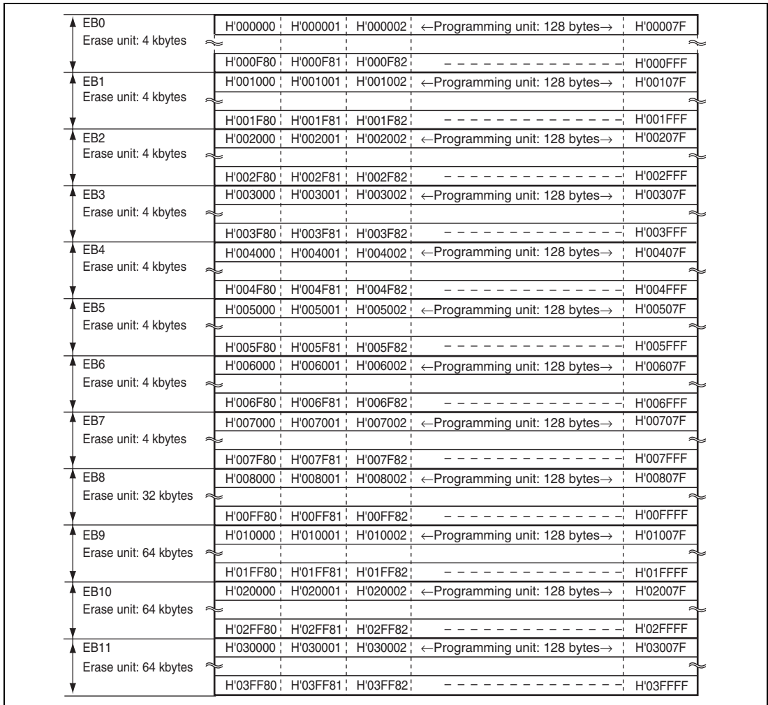
Figure 17.4 Block Structure of User MAT
