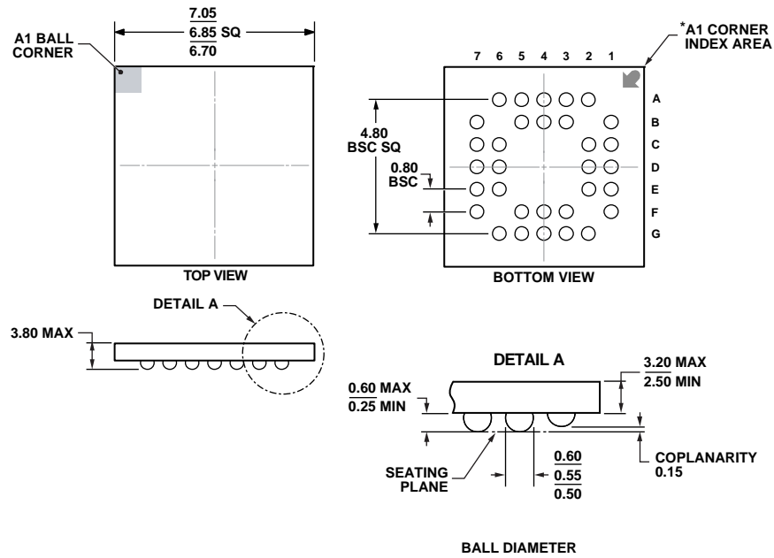
Figure 24. 32-Lead Ceramic Ball Grid Array [CBGA] (BC-32-3)
