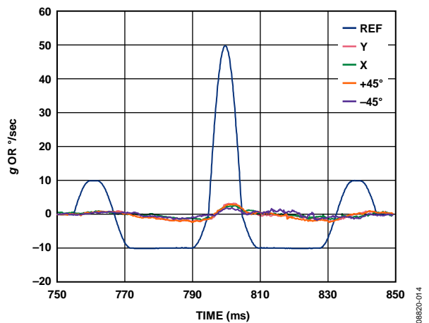
Figure 15. g and g \times g Sensitivity for a 50g, 10ms Pulse
