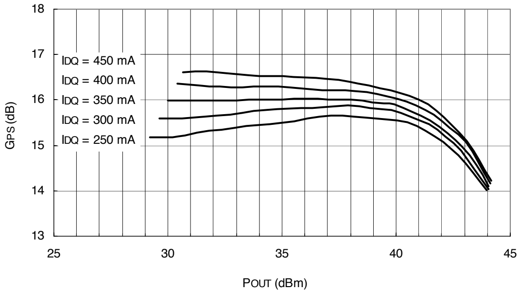
Figure 7. 2-Carrier N-CDMA Power Gain vs. Pout
