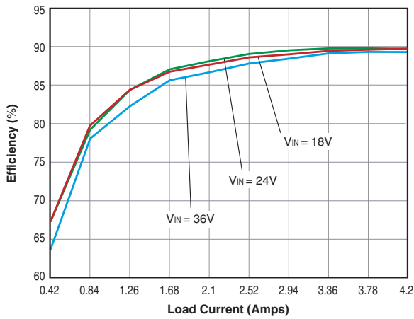
USQ-24/4.2-D24 Efficiency vs. Line Voltage/Load Current @ 25°C
