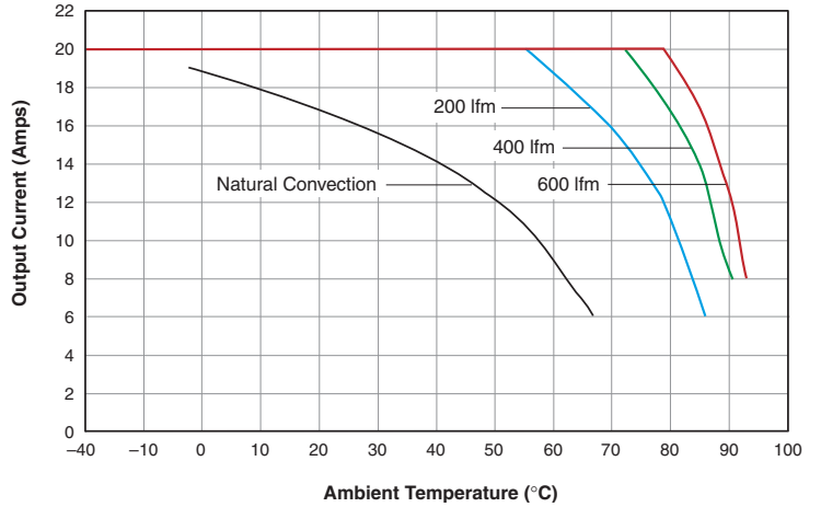
USQ-1.8/20-D48: Maximum Output Current vs. Ambient Temperature (Transverse air flow, pin 1 to pin 3; V IN = 48V, no heat sink.)
