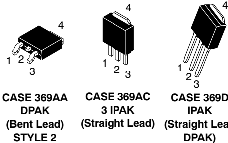
N-CHANNEL MOSFET
