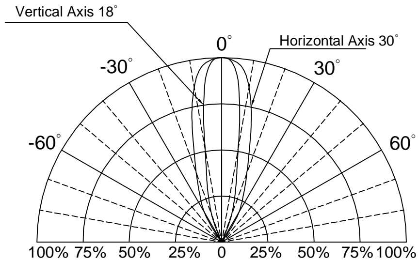
Radiation Angle(0.5):H 30 Degree/V 18 Degree
